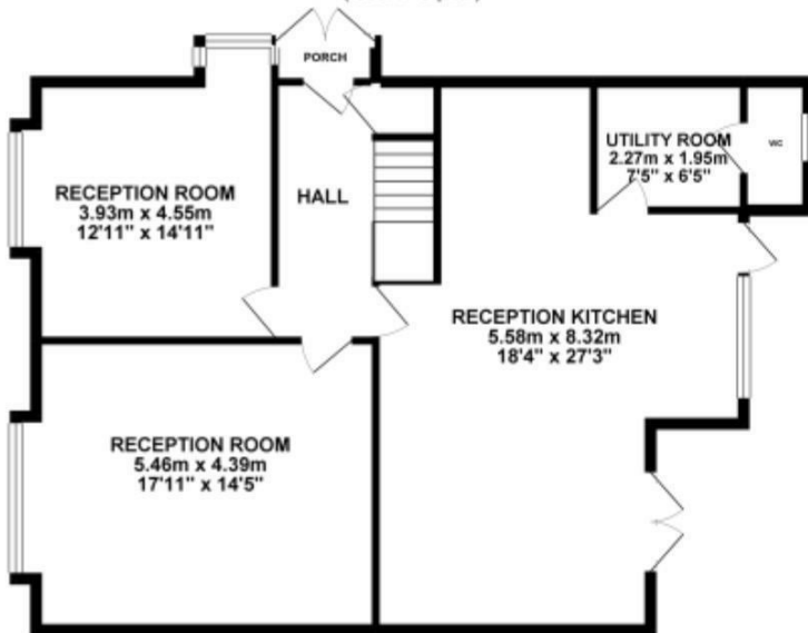
GROUND FLOOR 89.70 sq. m. (965.47 sq. ft.)
